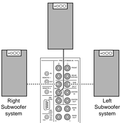
Subwoofer system
